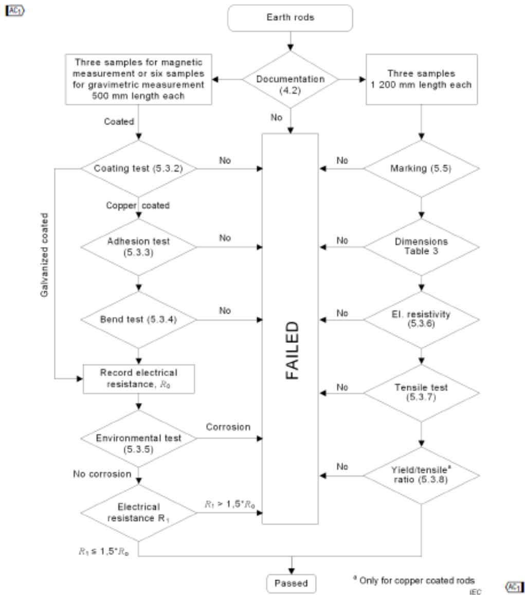
Figure F.1 – Flow chart of tests for earth rods
